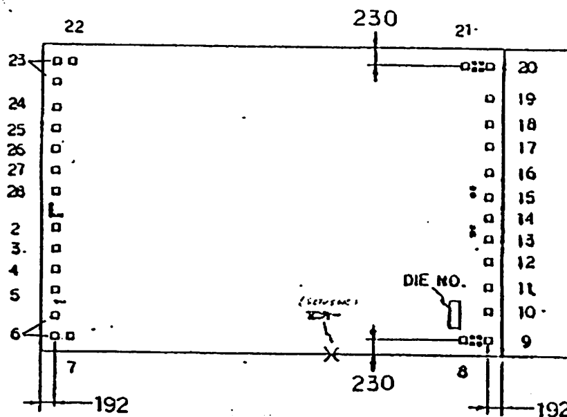
FIGURE 2 DIE CONFIGURATION
